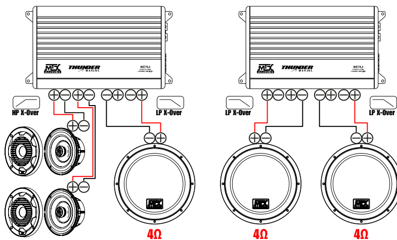
System diagram with 1 or 2 subwoofers
