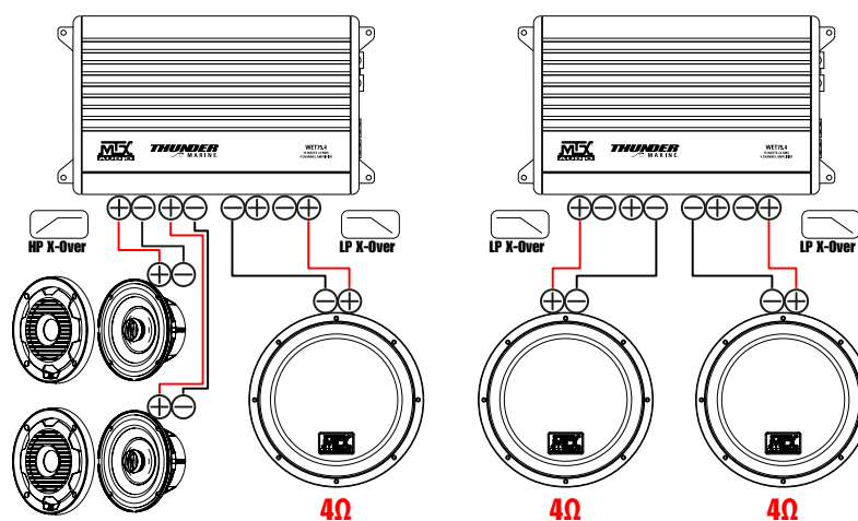
System diagram with 1 or 2 subwoofers
